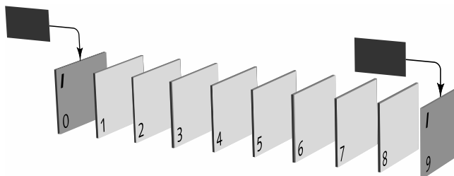
Figure 14.2 MPEG group of pictures (GOP) . The GOP depicted here has nine pictures, numbered 0 through 8. I-picture 0 is decoded from the coded data depicted in the dark gray block. Picture 9 is not in the GOP; it is the first picture of the next GOP. Here, the intra count ( n ) is 9.
