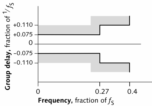
Figure 46.3 Filter template for Y' and R'G'B' components
