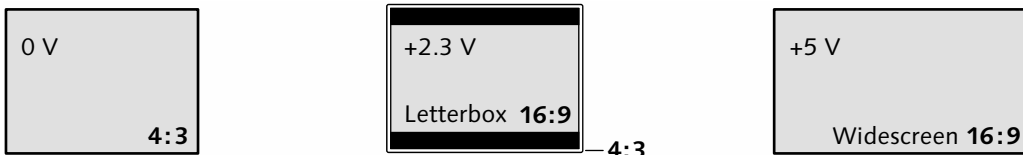
Figure 34.11 S-video widescreen signalling
