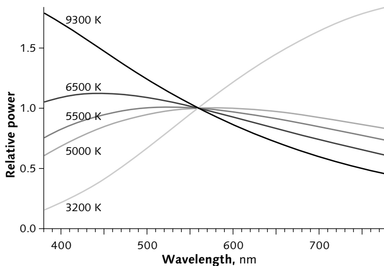
Figure 21.9 SPDs of blackbody radiators, normalized to equal power at 555 nm, are graphed here. The dramatically different spectral character of blackbody radiators at different temperatures is evident.
