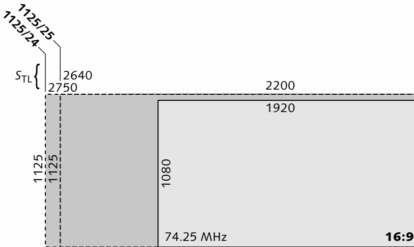
Figure 13.3 HDTV rasters at 24 Hz and 25 Hz carry an array of 1920 \times 1080 active samples, using a 74.25 MHz sampling rate at the interface. For 24 Hz (1080 p 24), the 1920 \times 1080 array is carried in an 1125/24 raster. For 25 Hz, the array is carried in an 1125/25 raster.
