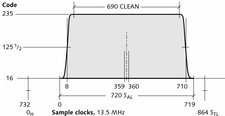
Figure 43.2 576i component digital 4:2:2 luma waveform
