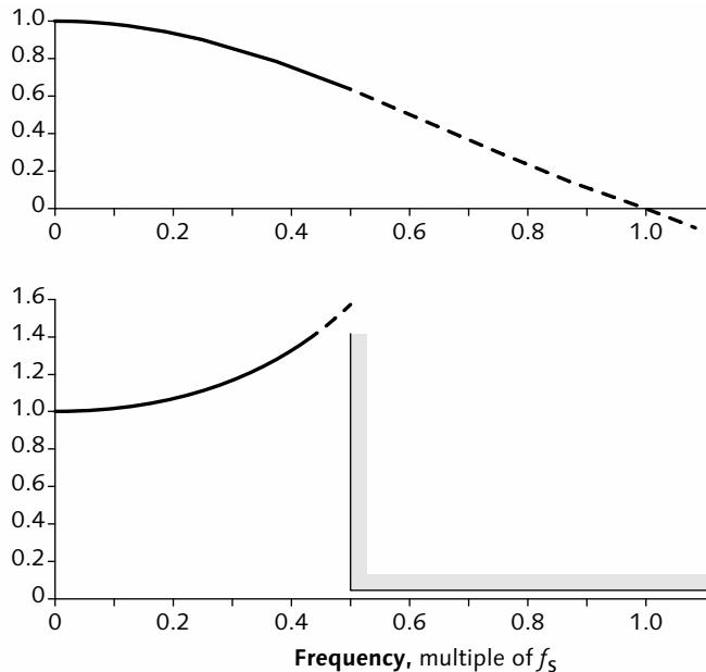
Figure 16.30 (sin x)/x correction is necessary following (or in principle, preceding) digital-to-analog conversion when a DAC with a typical boxcar output waveform is used. The frequency response of a boxcar-waveform DAC is shown in the upper graph. The lower graph shows the response of the (sin x)/x correction filter necessary to compensate its high frequency falloff.
