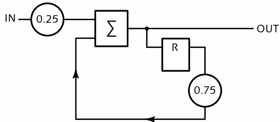
Figure 16.22 IIR ("recursive") filter computes a weighted sum of input samples (here, just \frac{1}{4} times the current sample), and adds to this a weighted sum of previous result samples. Every IIR filter exhibits nonlinear phase response.
