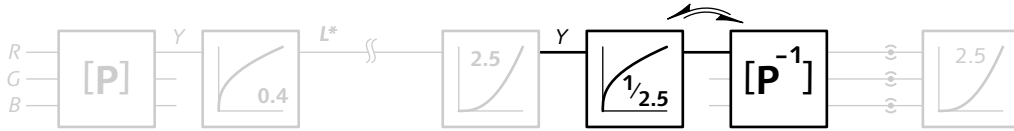
Figure 8.7 Rearranged decoder
