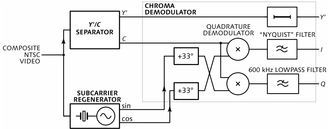
Figure 30.3 NTSC decoder using Y'IQ is similar to the decoder using Y'UV that I presented in Figure 28.5, on page 341. Phase shifts of 33° are applied to the sine and cosine phases of subcarrier. The Q lowpass filter has a corner of 600 kHz; the I lowpass filter has a special "Nyquist" shape detailed in Figure 30.4 overleaf. The 33° phase shifters and the Nyquist filter are useful only if the signal was encoded on [I, Q] axes with wideband I and narrowband Q. Because proper Y'IQ encoding has not been practiced since about 1970, using this textbook Y'IQ decoder is pointless.
