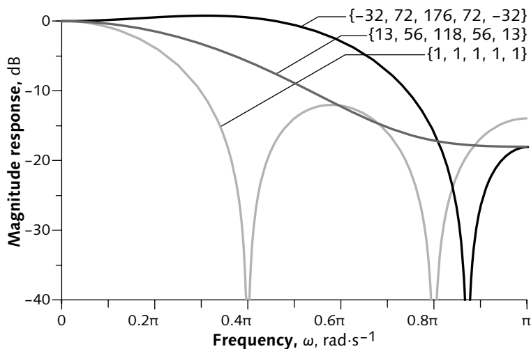
Figure 16.17 5-tap FIR filter responses are shown for several choices of coefficient values (tap weights).
