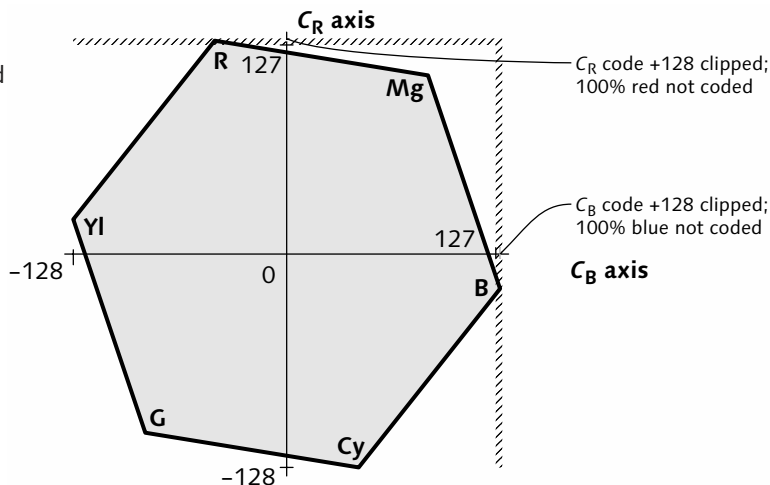
Figure 25.5 C_B C_R "full range" components used in JPEG/JFIF are shown, ranging from -128 to +127 . Chroma code +128 is clipped so that fully saturated blue and red cannot be preserved. No provision is made for undershoot or overshoot. The accompanying luma signal ranges 0 through 255.
