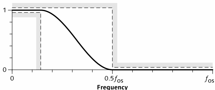
Figure 17.5 Analog filter for 2x-oversampling is much less demanding than a filter for direct sampling, because the difficult part of filtering – achieving a response comparable to that of Figure 17.4 – is relegated to the digital domain.
