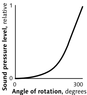
Figure 2.3 Audio taper
