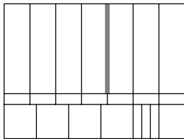
Figure 8.12 Failure to adhere to constant luminance is evident in the dark band in the green-magenta transition of the colorbar test signal.
