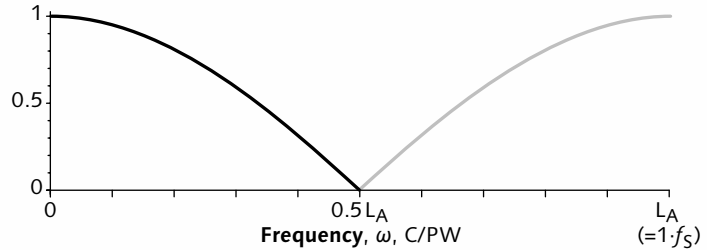
Figure 18.9 Response of [1, 1] FIR filter operating in the vertical domain, scaled for unity gain, is shown. This is a two-line ( 1H ) comb filter. Magnitude falls as \cos \omega .
