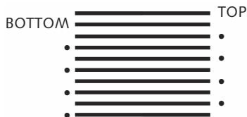
Figure 11.5 Interlacing in MPEG-2 identifies a picture according to whether it contains the top or bottom picture line of the frame. Top and bottom fields are displayed in the order that they are coded in an MPEG-2 data stream. For frame-coded pictures, display order is determined by a one-bit flag top field first , typically asserted for 576 i and negated for 480 i .
