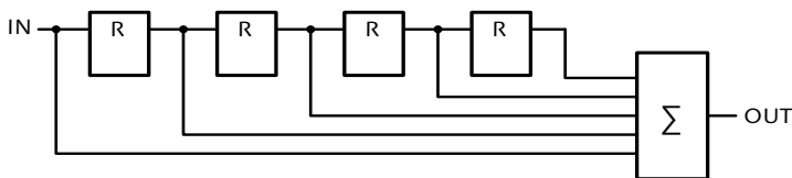
Figure 16.16 Block diagram of 5-tap FIR filter comprises four registers and an adder; five adjacent samples are summed. Prior to scaling to unity, the coefficients are [1, 1, 1, 1, 1].
