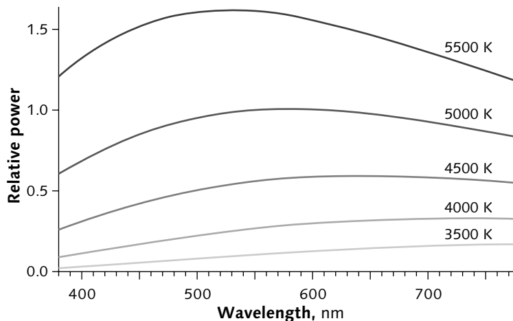
Figure 21.8 SPDs of blackbody radiators at several temperatures are graphed here. As the temperature increases, the absolute power increases and the peak of the spectral distribution shifts toward shorter wavelengths.
