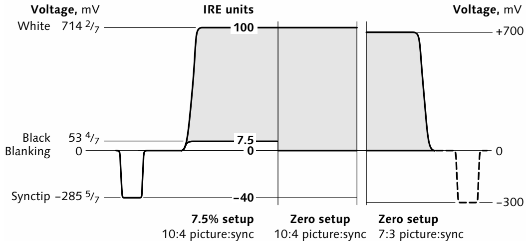
Figure 27.2 Comparison of 7.5% and zero setup. The left-hand third shows the video levels of composite 480 i video, with 7.5% setup and 10:4 picture-to-sync ratio. This coding is used in some studio equipment and in most computer monitor interfaces. The middle third shows zero setup and 10:4 picture-to-sync, as used in 480 i video in Japan. EBU N10 component video, 576 i systems, and HDTV use zero setup, 700 mV picture, and 300 mV sync, as shown at the right.
