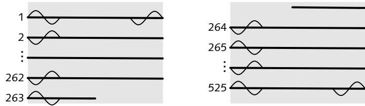
Figure 29.4 Color subcarrier in NTSC has its frequency chosen so that subcarrier phase inverts line-to-line. If U and V color difference components are constant line-to-line, then the phase of modulated chroma will invert line-to-line; this enables a comb filter to separate luma and chroma. A field comprises an odd integer number of halflines; it contains an odd integer number of half-cycles of subcarrier. Thus, subcarrier inverts phase frame-to-frame. This leads to NTSC color-frames A and B .
