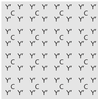
Figure 10.2 Subsampling schemes are summarized here. C indicates a [ C_B , C_R ] sample pair when located at the same site; otherwise (as in the DV schemes) individual C_B and C_R notations indicate the centers of the respective chroma samples. Y' indicates the center of a luma sample. The schemes in the left column are progressive. The schemes in the right column are interlaced; there, black letters indicate top field samples and gray letters indicate bottom field samples.
