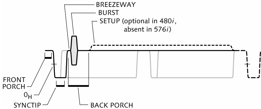
Figure 34.5 Sync features
