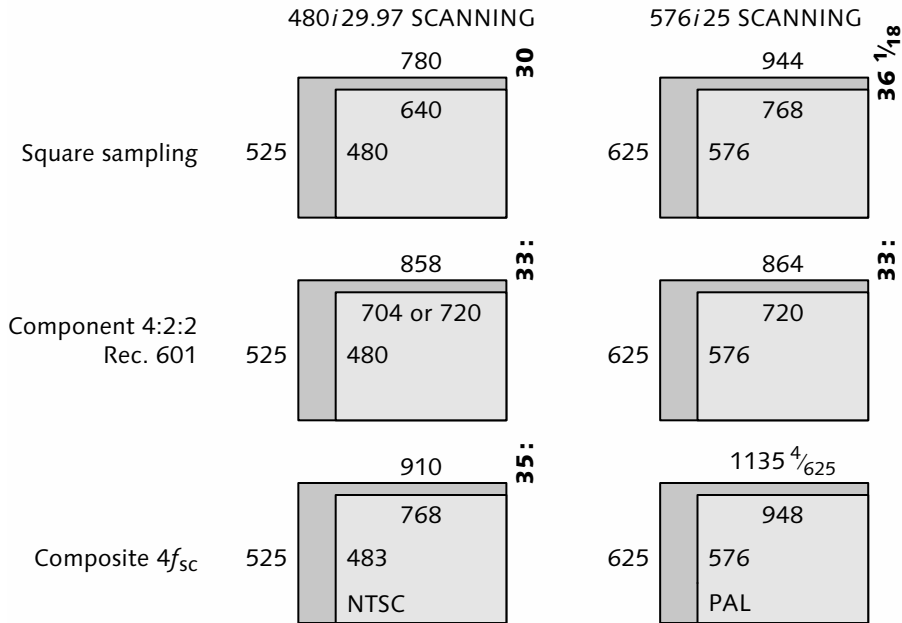
Figure 11.1 SDTV digital video raster s for 4:3 aspect ratio. 480i29.97 scanning is at the left, 576i25 at the right. The top row shows square sampling ("square pixels"). The middle row shows sampling at the Rec. 601 standard sampling frequency of 13.5 MHz. The bottom row shows sampling at four times the color subcarrier frequency ( 4f_{sc} ). Above each diagram is its count of samples per total line ( S_{TL} ); ratios among S_{TL} values are written vertically in bold numerals.
