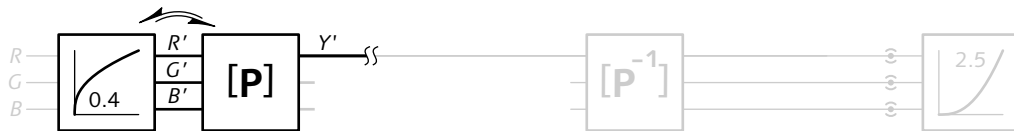
Figure 8.9 Rearranged encoder
