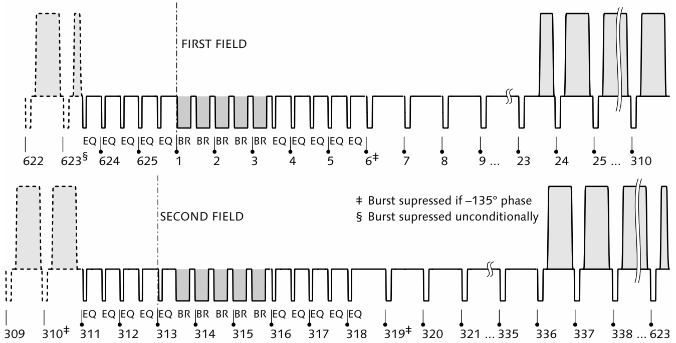
Figure 43.1 576i raster, vertical. This drawing shows waveforms of first and second fields, detailing vertical sync intervals. The first field comprises 312 lines, and the second field comprises 313 lines.
