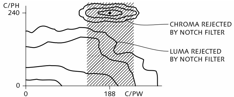
Figure 29.14 Spatial frequency response of NTSC "notch" filter shows that a large portion of the luma spectrum is wrongly decoded as chroma. In areas of fine periodic luma detail, cross-color artifacts such as swirling color rainbows are liable to appear.
