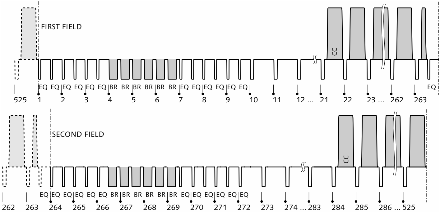
Figure 41.1 480i raster, vertical. This drawing shows waveforms of first and second fields, detailing the vertical sync intervals. CC indicates a line that may contain EIA 608 ("line 21") closed caption data.
