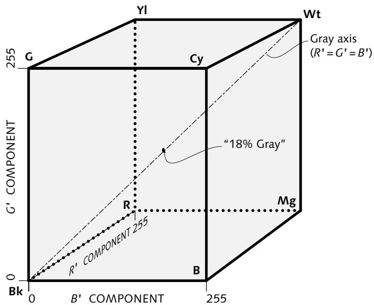
Figure 24.1 RGB and R'G'B' cubes . RGB components form the coordinates of a three-dimensional color space; coordinate values between 0 and 1 define the unit cube. Linear coding, sketched at the top, has poor perceptual performance. In video, RGB components are subject to gamma correction ; this yields perceptually uniform R'G'B' that exhibits good performance with 8-bit components.
