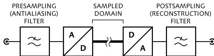
Figure 16.27 Sampling and reconstruction
