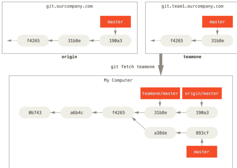
FIGURE 3-26 Remote tracking branch for teamone/ master
