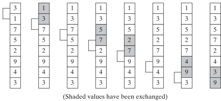
FIGURE 9-4 First pass through an array (bubble sort).
