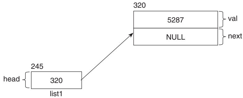
Figure 9.21 Observed effect of the appendNode() function
