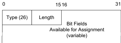
Figure 8-60 The Router Advertisement Expanded Flags option provides an arbitrary amount of additional space for defining future RA flags.
