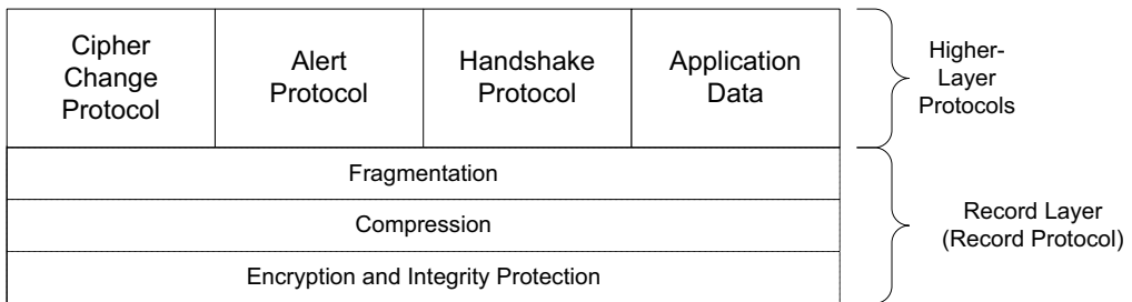
Figure 18-28 The TLS protocol “stack” has a lower record layer and three of its own upper-layer protocols called handshaking protocols. A fourth upper-layer protocol is the application protocol using TLS. The record layer provides fragmentation, compression, integrity protection, and encryption. The handshaking protocols perform many of the same tasks for TLS that IKE does for IPsec.
