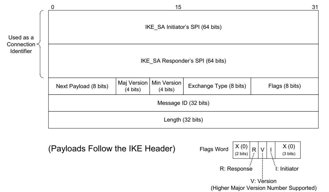
Figure 18-11 The IKE v2 header. All IKE messages contain a header followed by zero or more payloads. IKE uses 64-bit SPI values. The Exchange Type gives the purpose of the exchange and the payloads that may be expected in the message. The Flags field indicates whether the message was sent from an initiator or a responder. The Message ID associates requests with responses and is used for detecting replay attacks.
