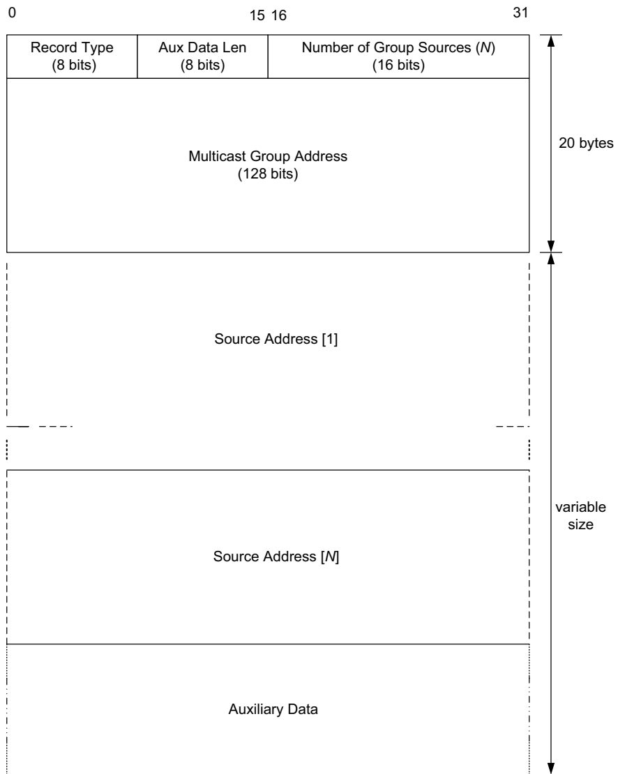
Figure 8-29 A multicast address (group) record. Multiple such records may be present in an MLDv2 Report message. The Record Type field is one of the following: MODE_IS_INCLUDE , MODE_IS_EXCLUDE , CHANGE_TO_INCLUDE_MODE , CHANGE_TO_EXCLUDE_MODE , ALLOW_NEW_SOURCES , or BLOCK_OLD_SOURCES . LW-MLDv2 simplifies MLDv2 by removing the EXCLUDE modes. The Aux Data Len field contains the amount of auxiliary data present in the record, in 32-bit-word units. For MLDv2, as specified in [RFC3810], this field must contain the value 0, indicating no auxiliary data.
